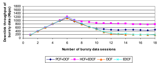
Fig. 10: Downlink throughput of bursty data streams.
